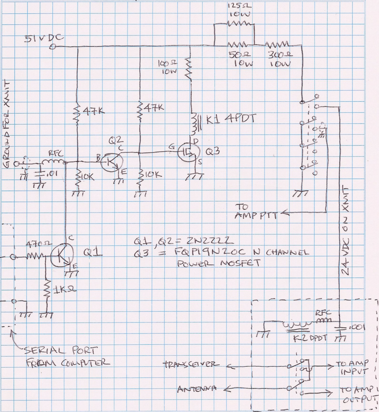
COAXIAL RELAY (HOME BUILT)
