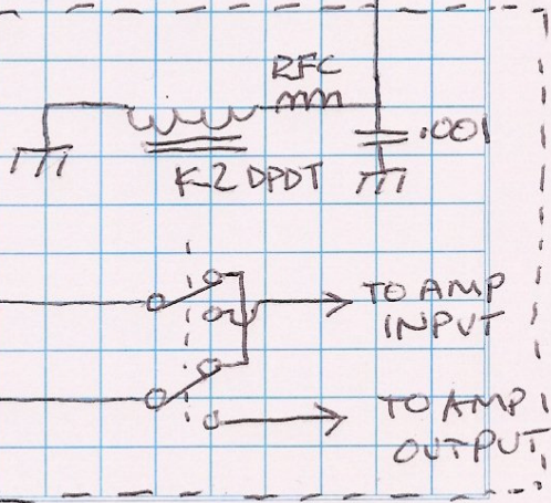
COAXIAL RELAY (HOME BUILT)
